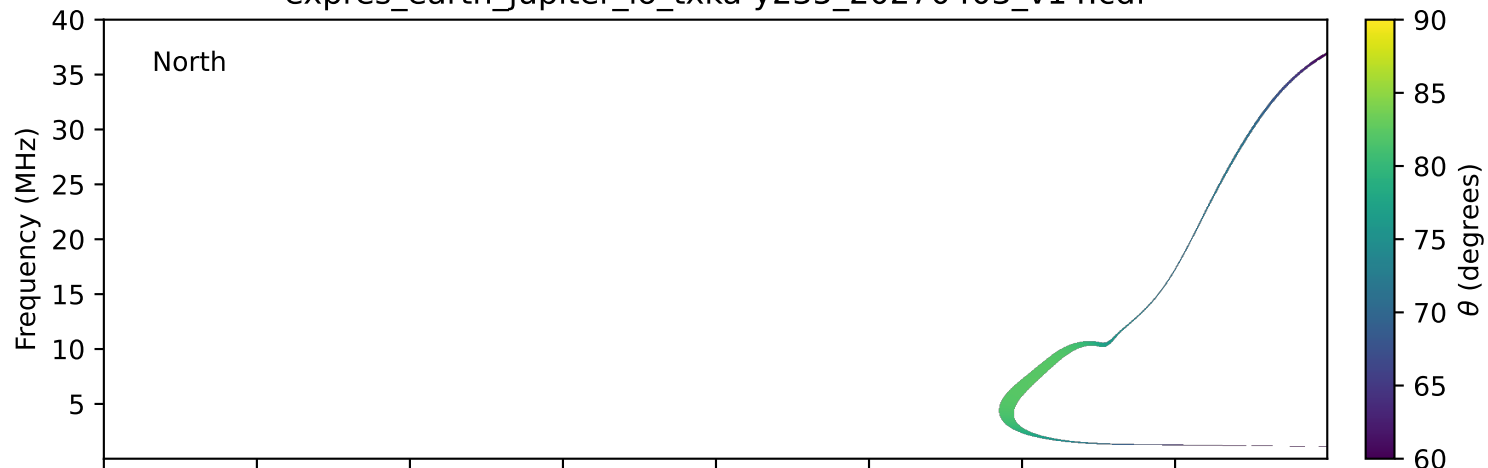
expres_earth_jupiter_io_txka-y235_20270403_v14.cdf
