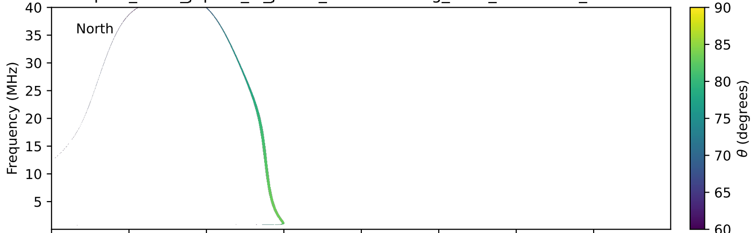
expres_earth_jupiter_io_jrm33_lossc-wid1deg_3kev_20270413_v11.cdf
