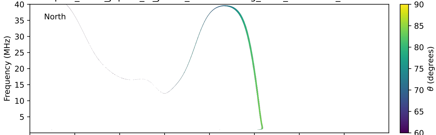
expres_earth_jupiter_io_jrm33_lossc-wid1deg_3kev_20270411_v11.cdf
