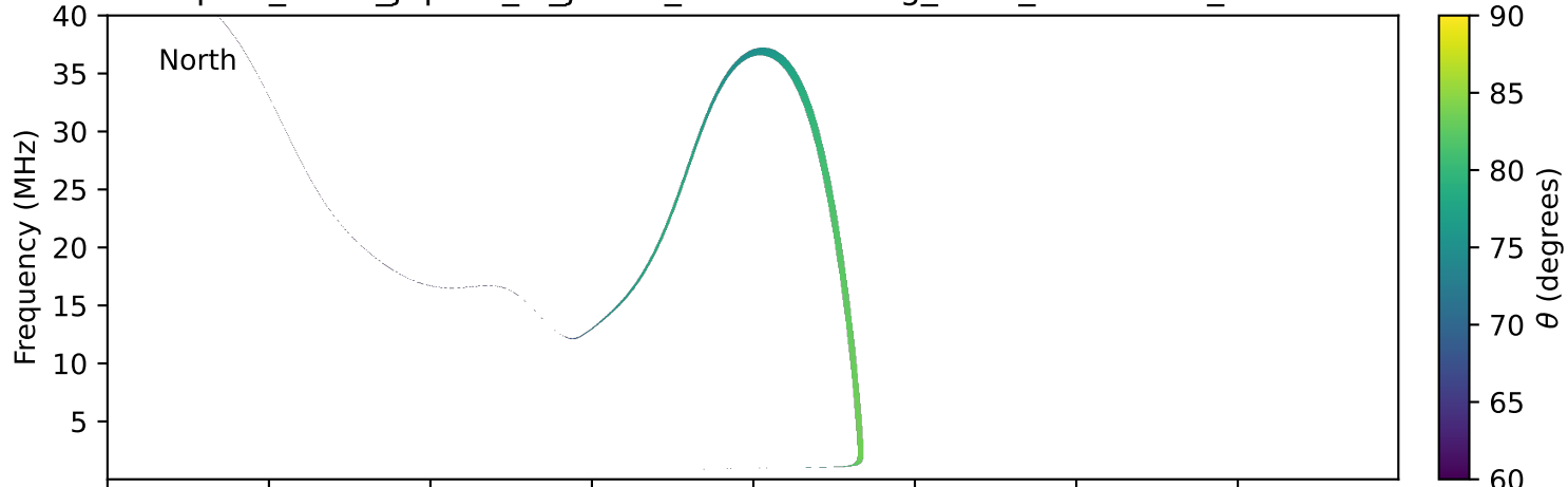
expres_earth_jupiter_io_jrm33_lossc-wid1deg_3kev_20270404_v11.cdf
