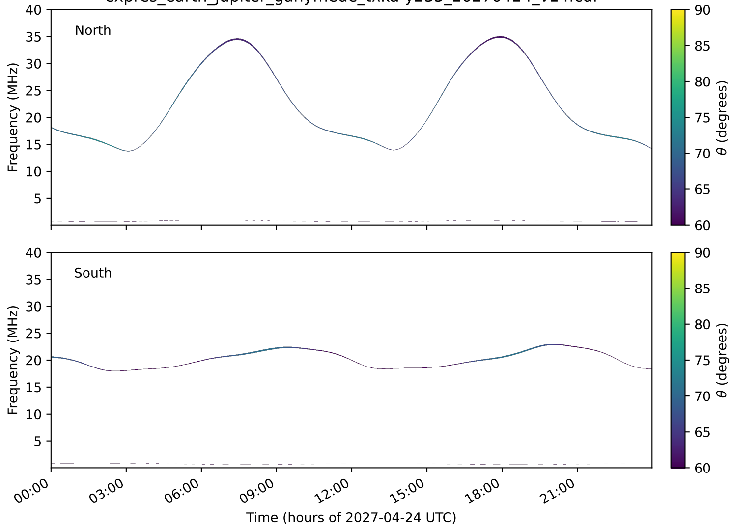
expres_earth_jupiter_ganymede_txka-y235_20270424_v14.cdf
