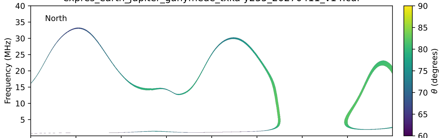
expres_earth_jupiter_ganymede_txka-y235_20270411_v14.cdf
