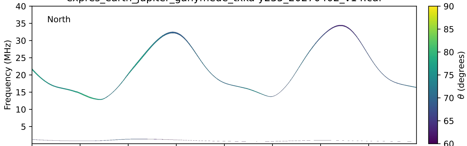
expres_earth_jupiter_ganymede_txka-y235_20270402_v14.cdf
