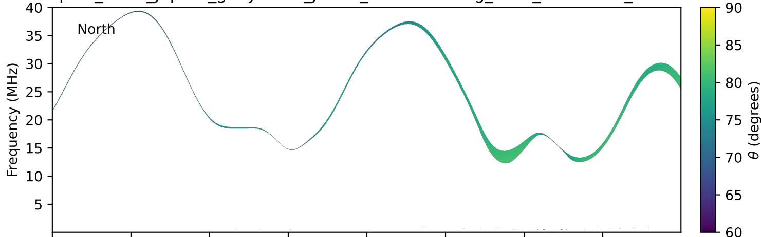
expres_earth_jupiter_ganymede_jrm33_lossc-wid1deg_3kev_20270411_v11.cdf
