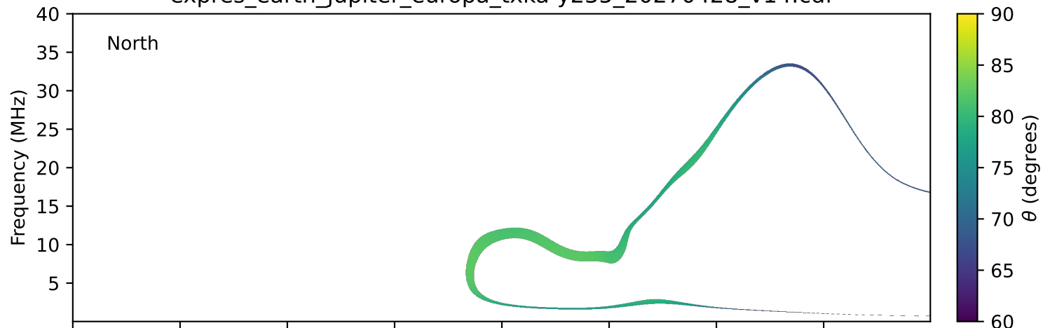
expres_earth_jupiter_europa_txka-y235_20270428_v14.cdf
