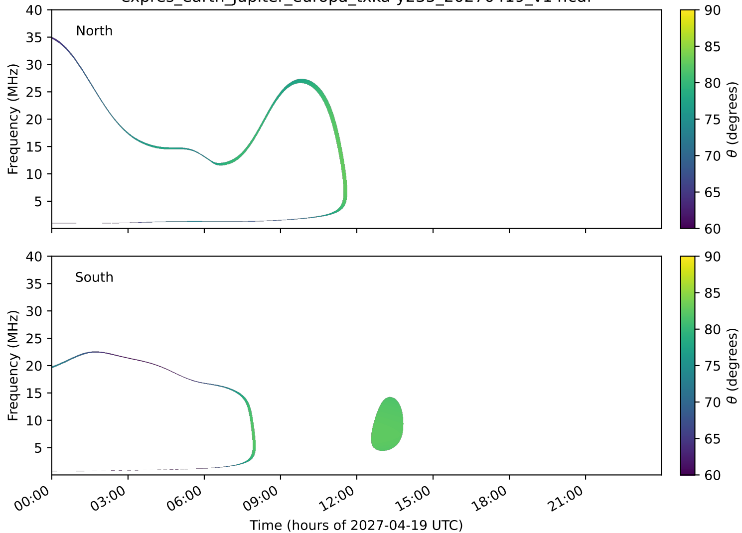
expres_earth_jupiter_europa_txka-y235_20270419_v14.cdf
