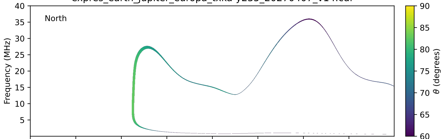
expres_earth_jupiter_europa_txka-y235_20270407_v14.cdf
