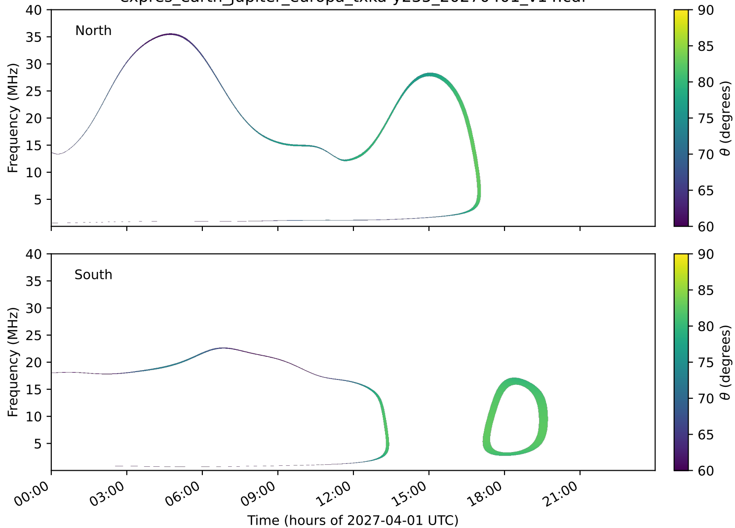
expres_earth_jupiter_europa_txka-y235_20270401_v14.cdf
