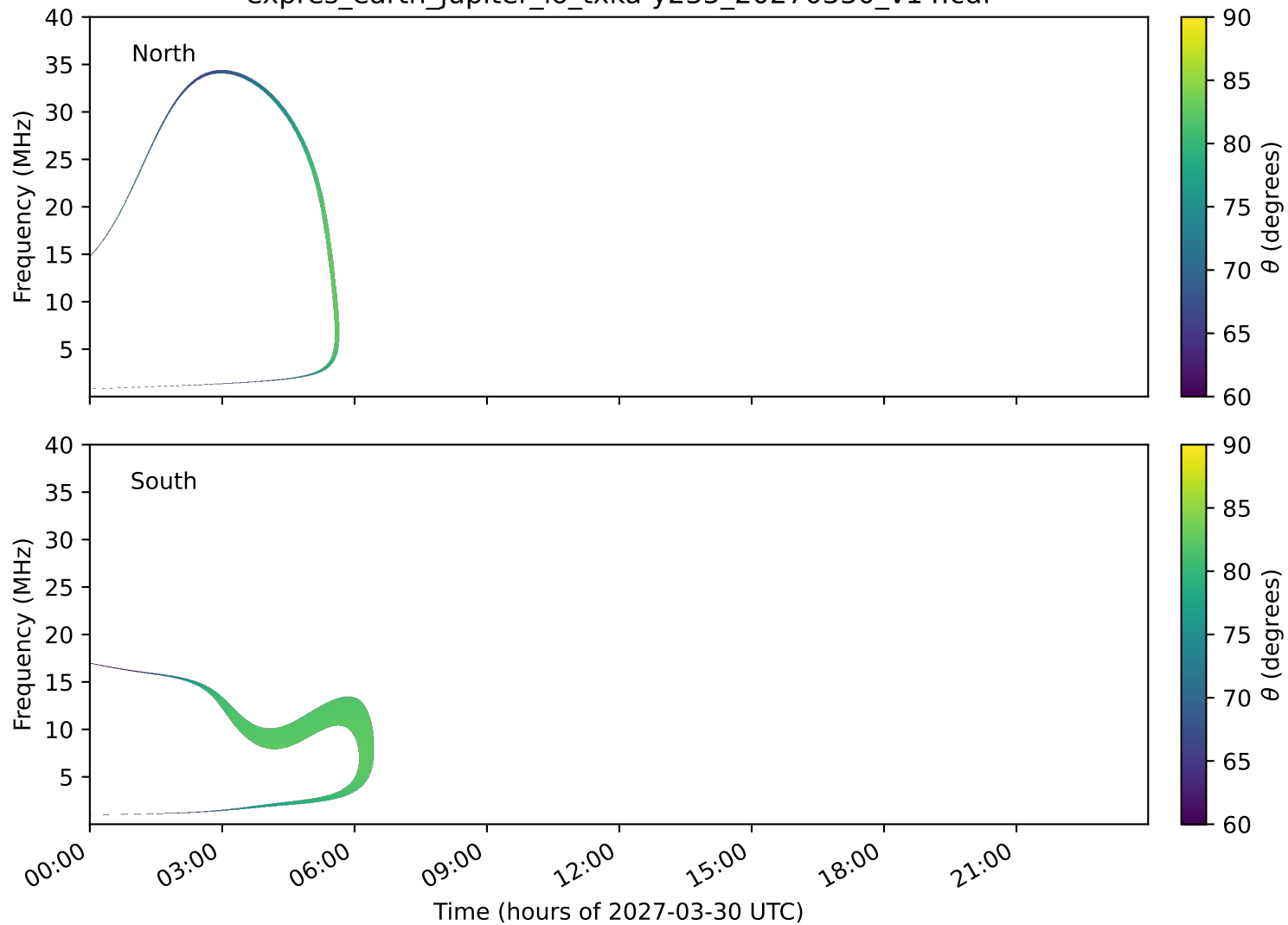
expres_earth_jupiter_io_txka-y235_20270330_v14.cdf
