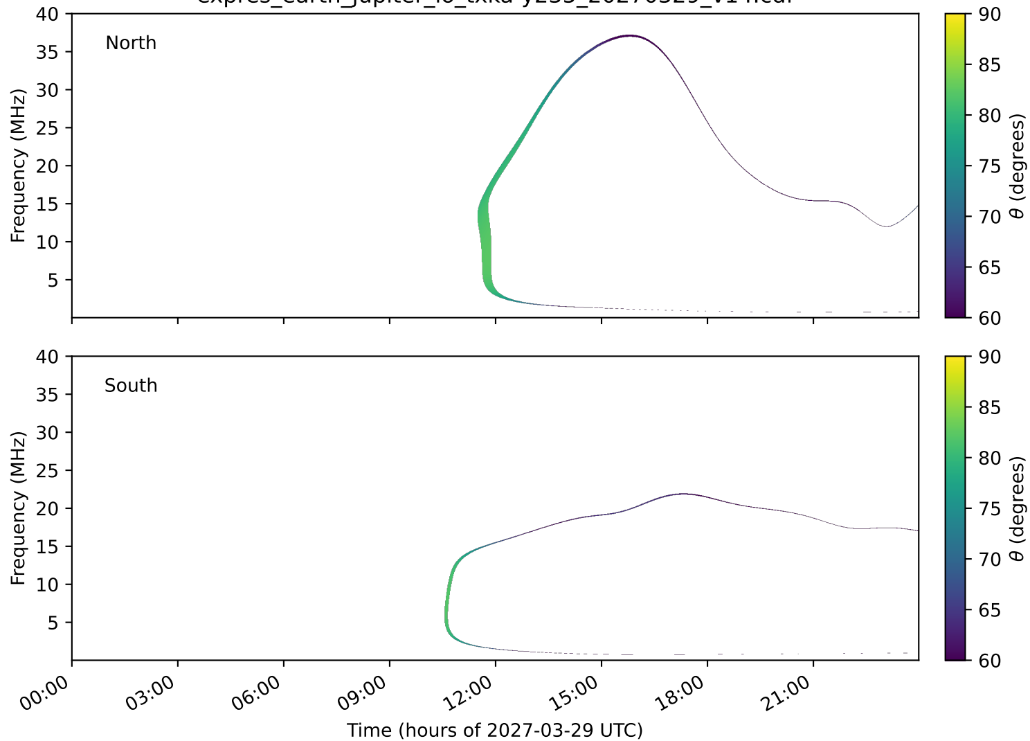
expres_earth_jupiter_io_txka-y235_20270329_v14.cdf
