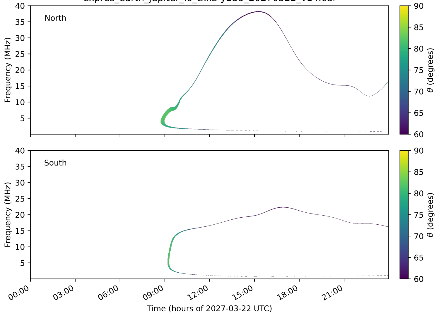
expres_earth_jupiter_io_txka-y235_20270322_v14.cdf
