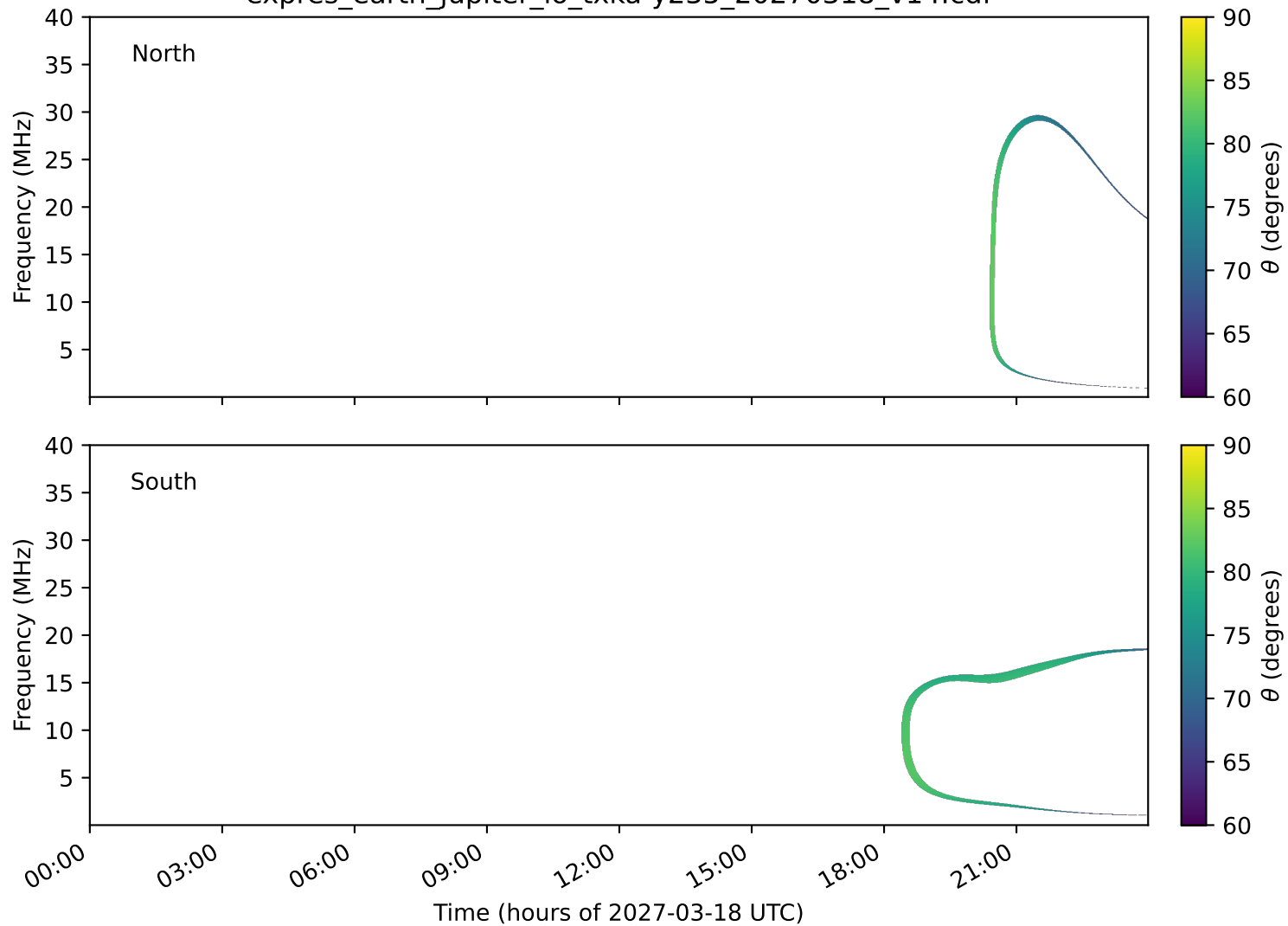
expres_earth_jupiter_io_txka-y235_20270318_v14.cdf
