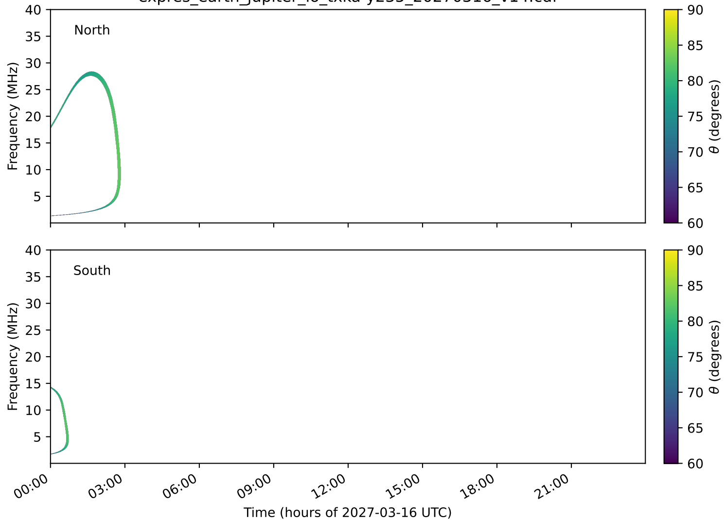
expres_earth_jupiter_io_txka-y235_20270316_v14.cdf
