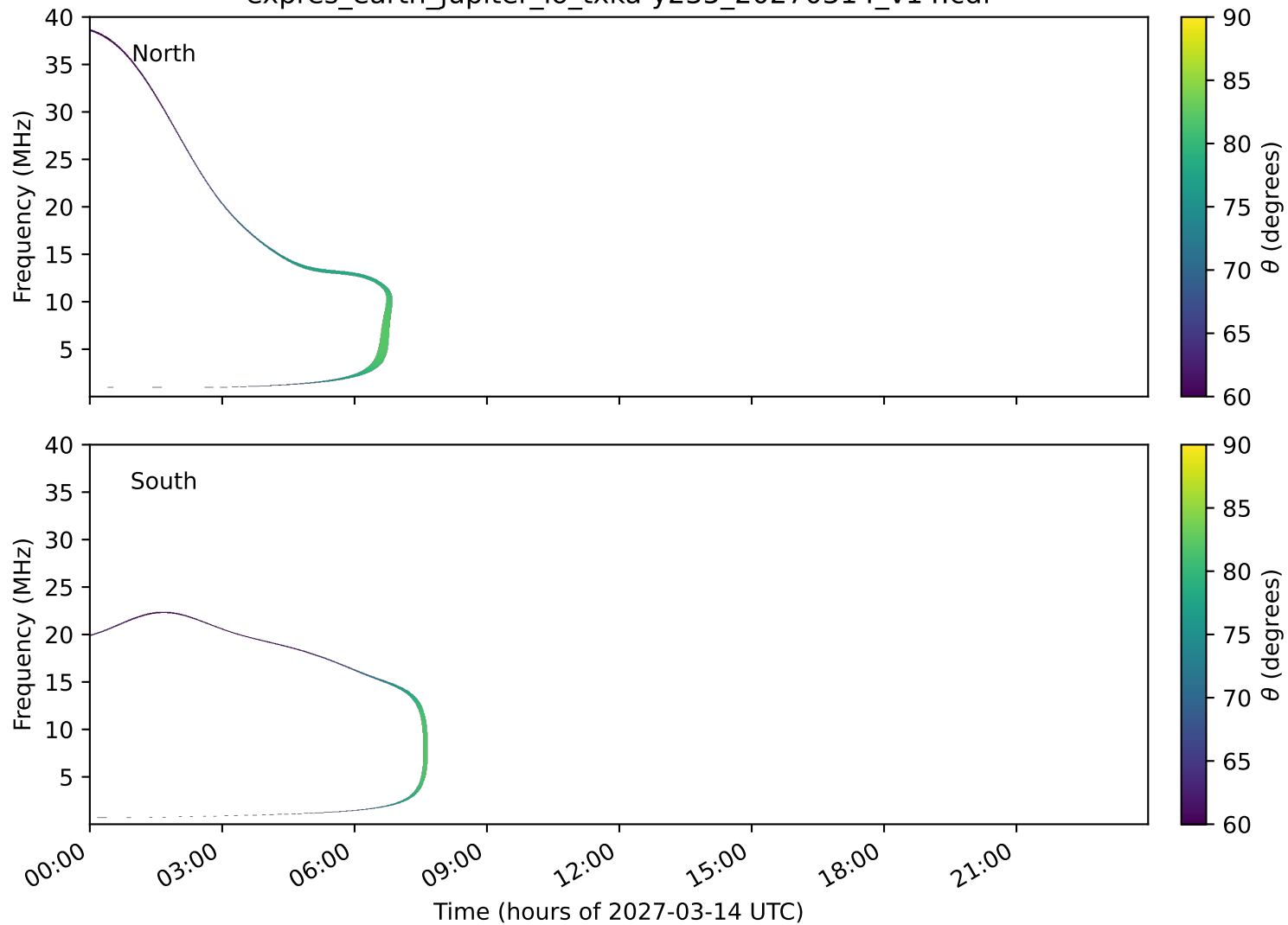
expres_earth_jupiter_io_txka-y235_20270314_v14.cdf
