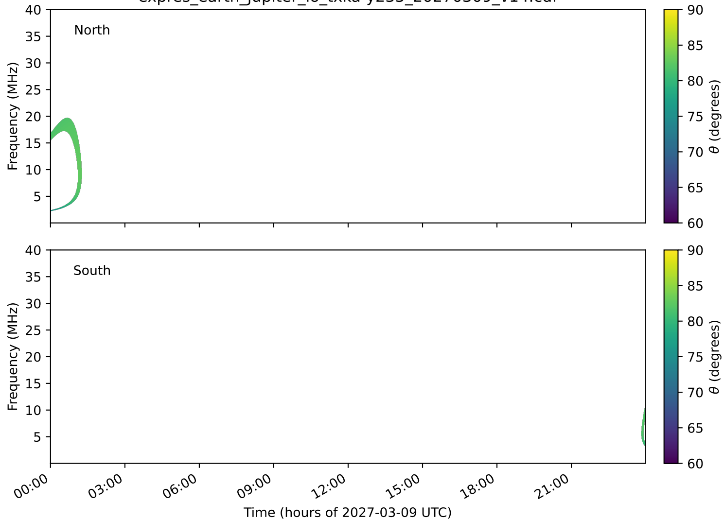
expres_earth_jupiter_io_txka-y235_20270309_v14.cdf
