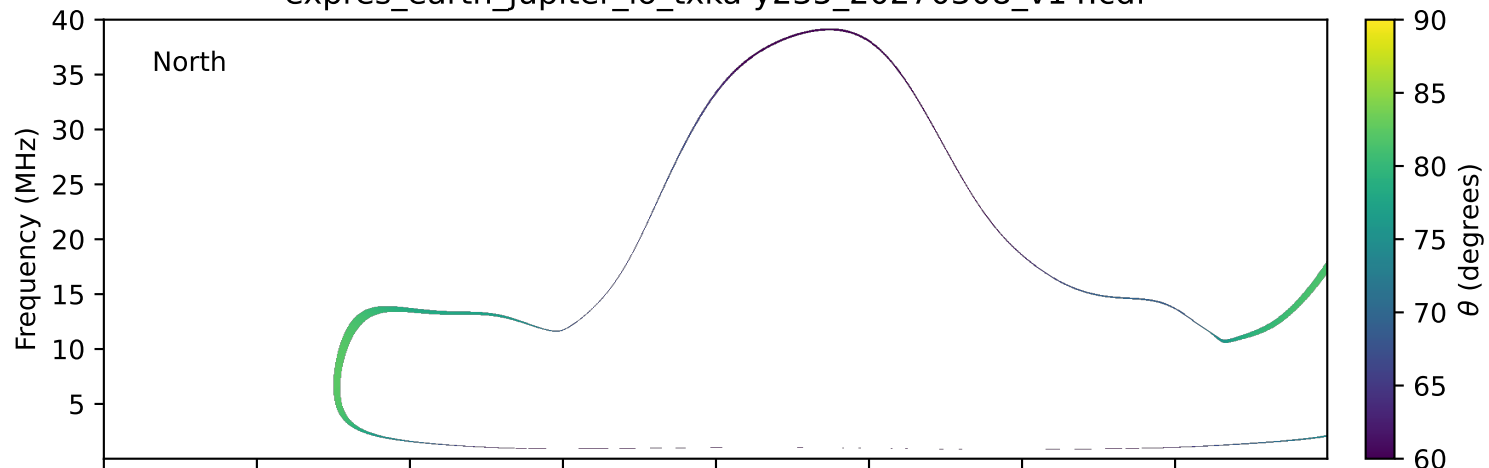
expres_earth_jupiter_io_txka-y235_20270308_v14.cdf
