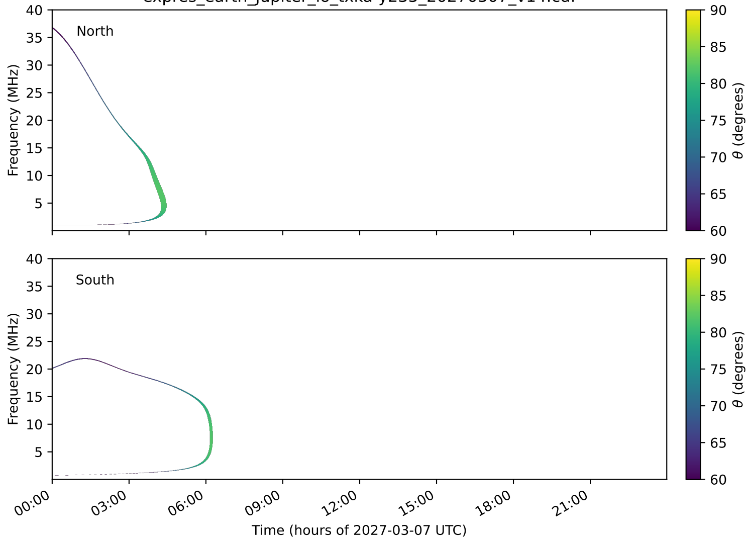
expres_earth_jupiter_io_txka-y235_20270307_v14.cdf
