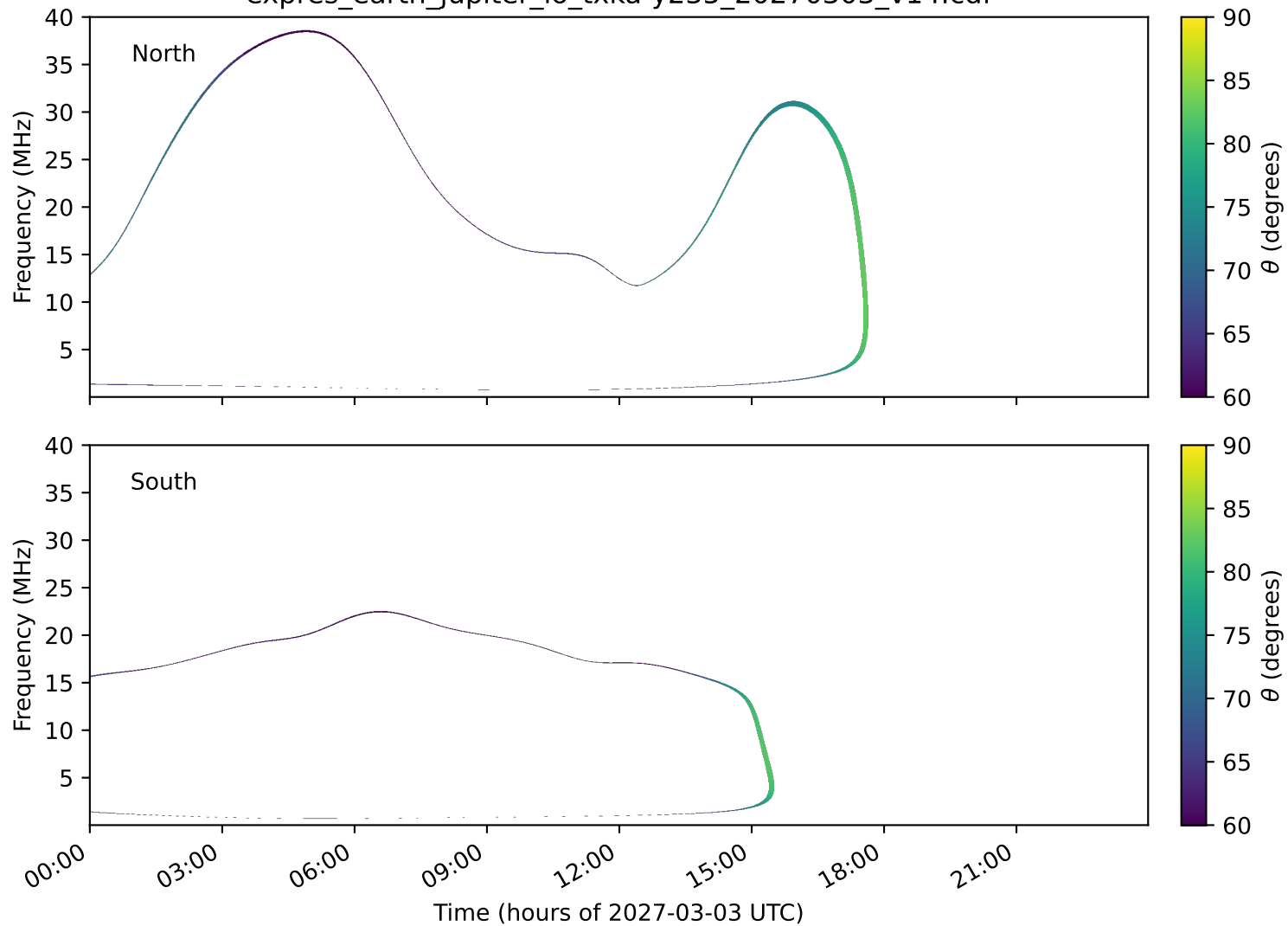
expres_earth_jupiter_io_txka-y235_20270303_v14.cdf
