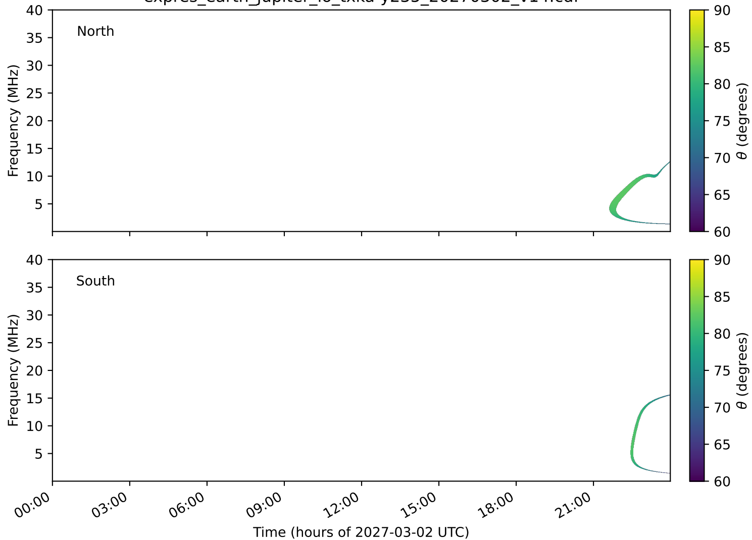
expres_earth_jupiter_io_txka-y235_20270302_v14.cdf
