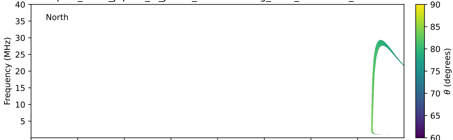
expres_earth_jupiter_io_jrm33_lossc-wid1deg_3kev_20270325_v11.cdf
