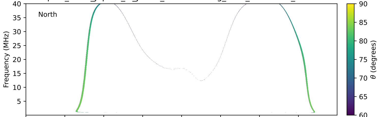
expres_earth_jupiter_io_jrm33_lossc-wid1deg_3kev_20270324_v11.cdf
