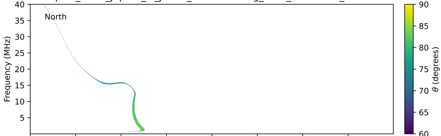
expres_earth_jupiter_io_jrm33_lossc-wid1deg_3kev_20270314_v11.cdf
