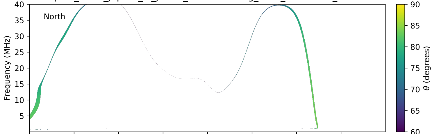
expres_earth_jupiter_io_jrm33_lossc-wid1deg_3kev_20270310_v11.cdf
