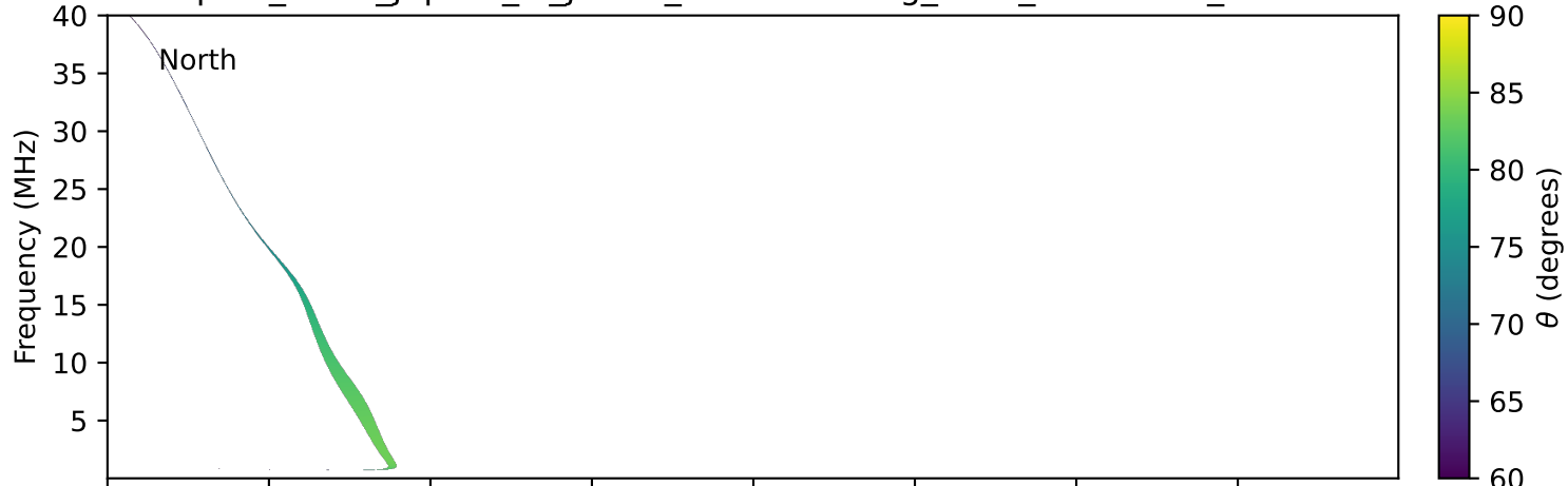
expres_earth_jupiter_io_jrm33_lossc-wid1deg_3kev_20270307_v11.cdf
