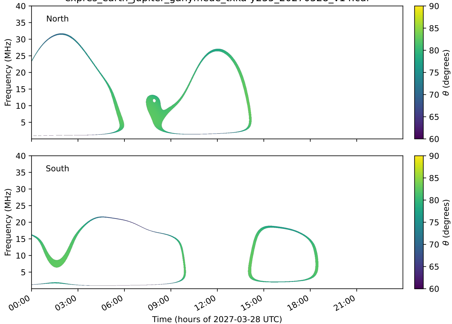
expres_earth_jupiter_ganymede_txka-y235_20270328_v14.cdf
