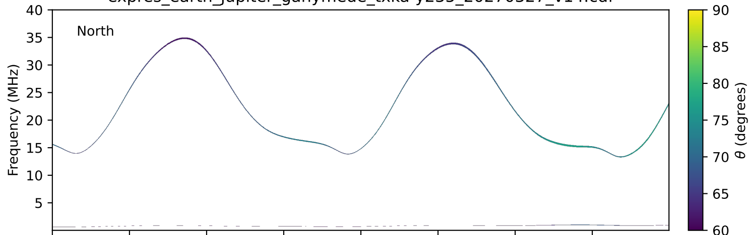
expres_earth_jupiter_ganymede_txka-y235_20270327_v14.cdf
