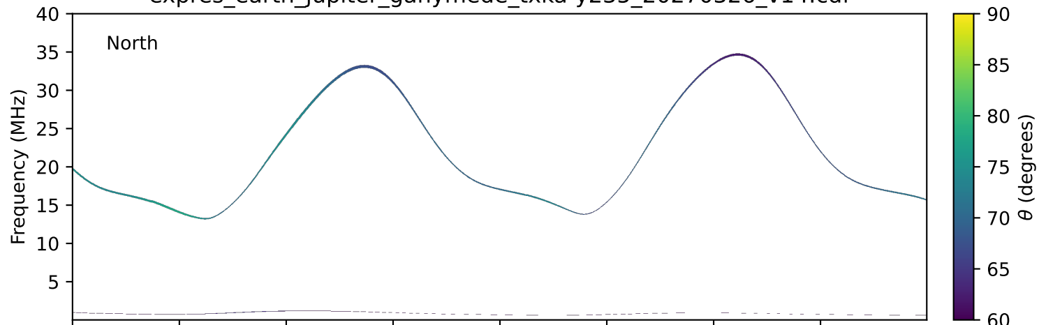
expres_earth_jupiter_ganymede_txka-y235_20270326_v14.cdf
