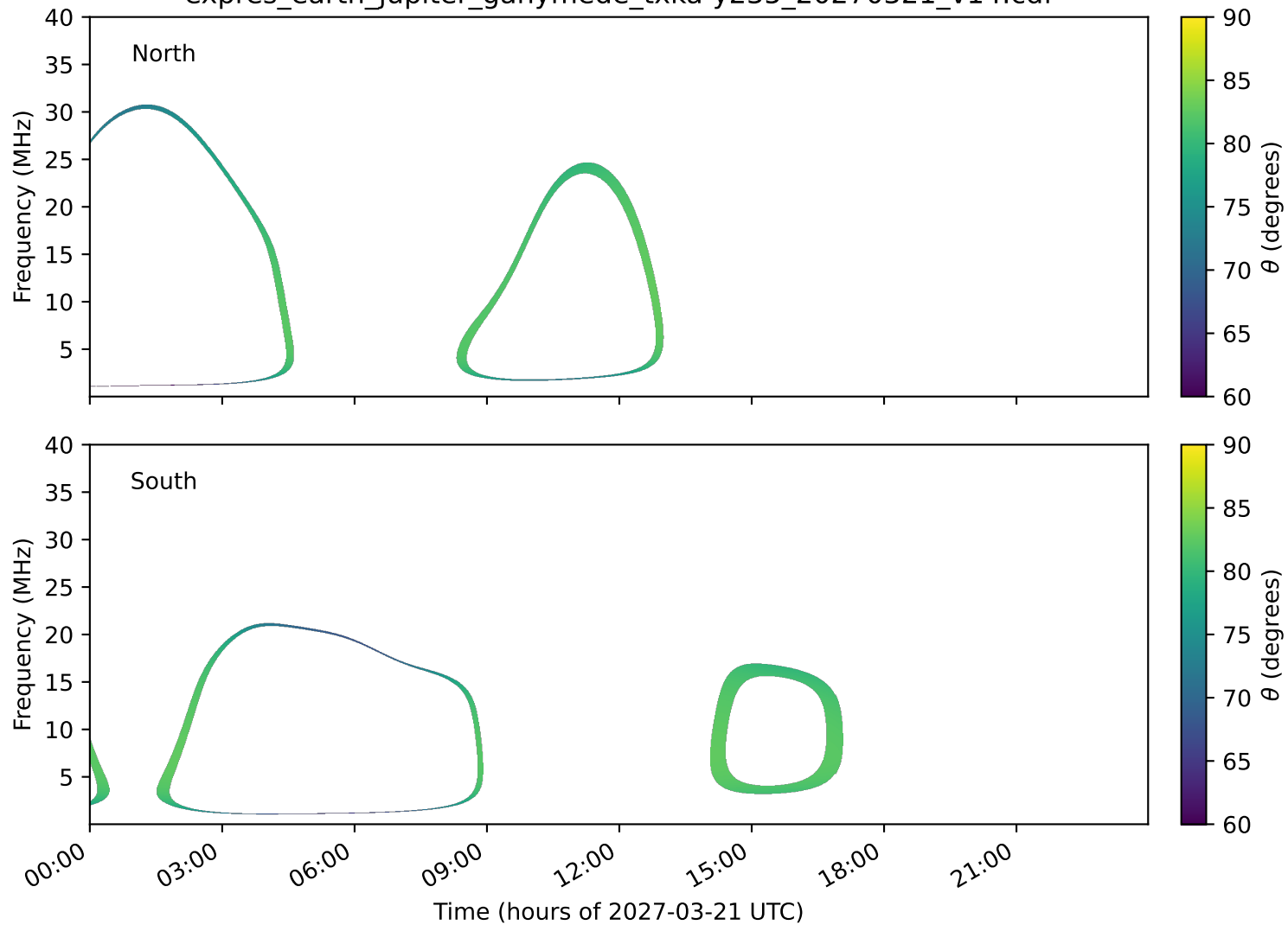
expres_earth_jupiter_ganymede_txka-y235_20270321_v14.cdf
