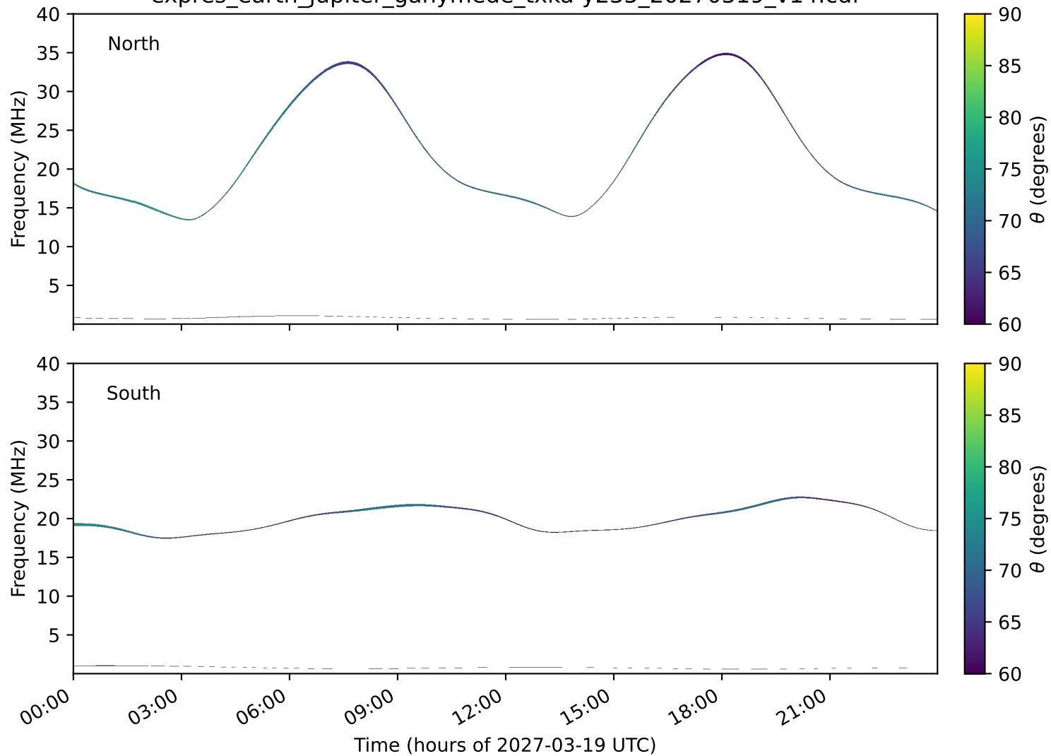
expres_earth_jupiter_ganymede_txka-y235_20270319_v14.cdf
