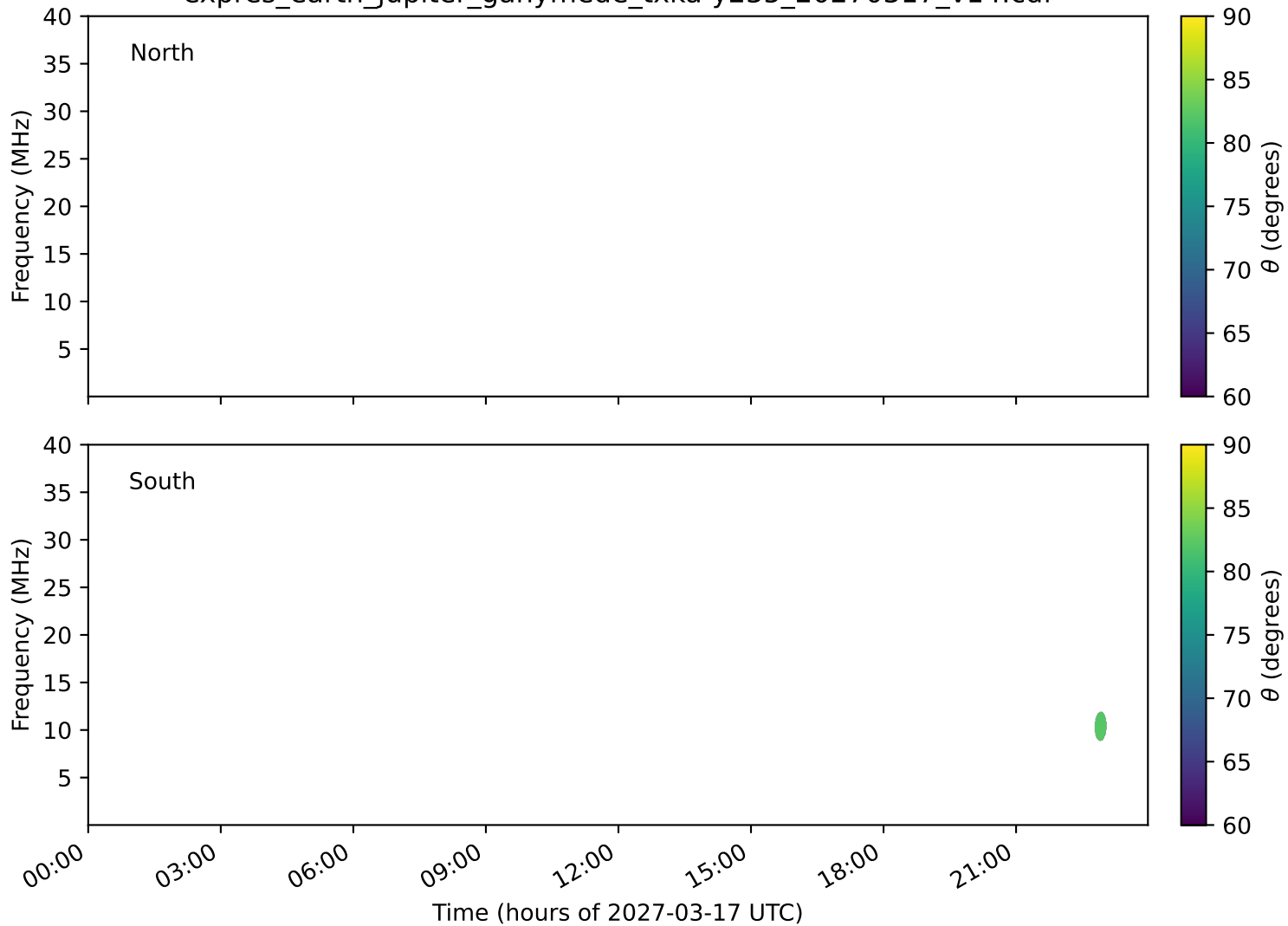
expres_earth_jupiter_ganymede_txka-y235_20270317_v14.cdf
