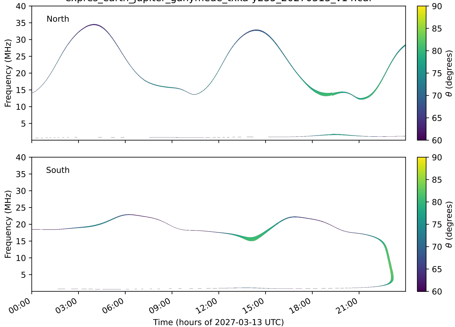
expres_earth_jupiter_ganymede_txka-y235_20270313_v14.cdf
