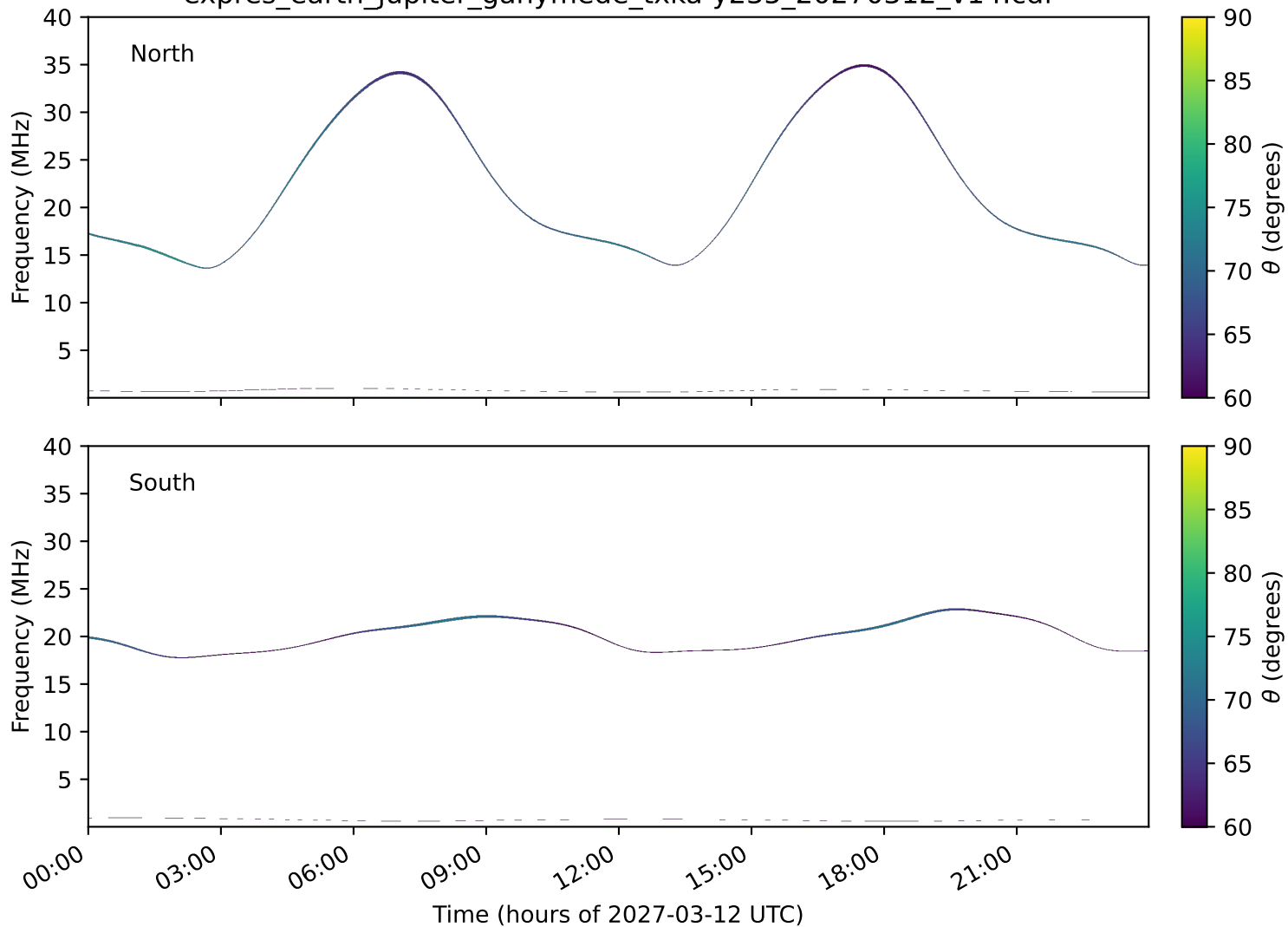
expres_earth_jupiter_ganymede_txka-y235_20270312_v14.cdf
