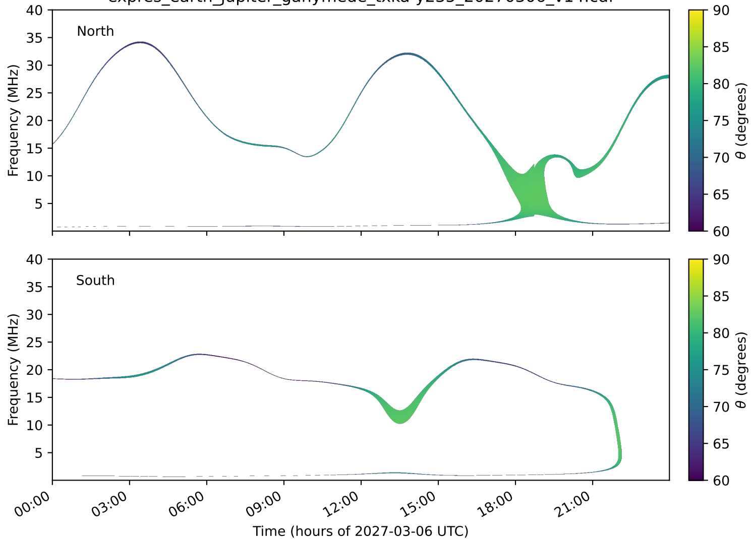
expres_earth_jupiter_ganymede_txka-y235_20270306_v14.cdf
