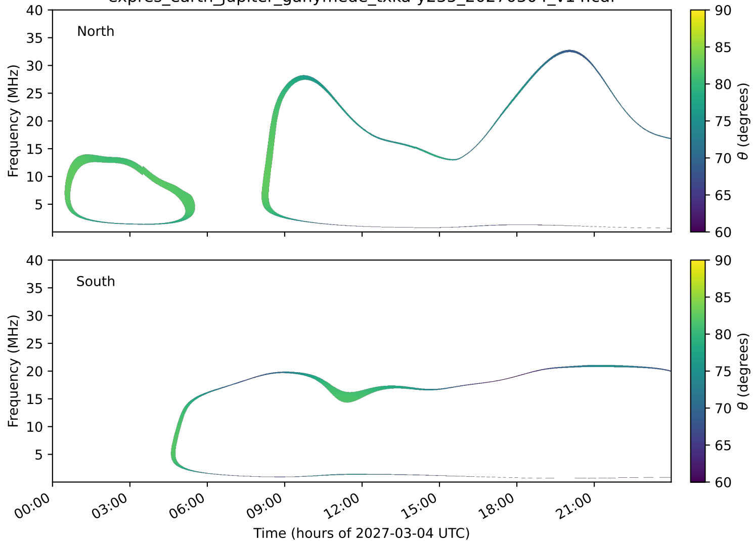
expres_earth_jupiter_ganymede_txka-y235_20270304_v14.cdf
