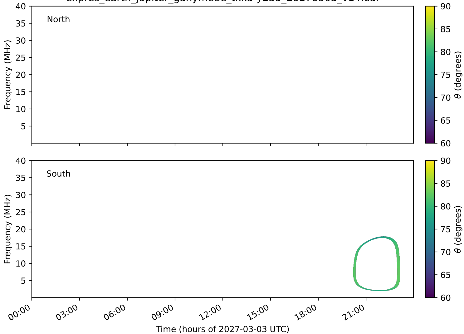
expres_earth_jupiter_ganymede_txka-y235_20270303_v14.cdf
