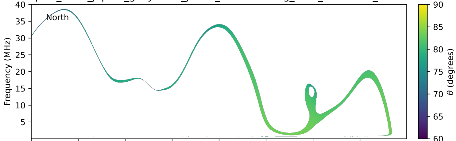
expres_earth_jupiter_ganymede_jrm33_lossc-wid1deg_3kev_20270328_v11.cdf
