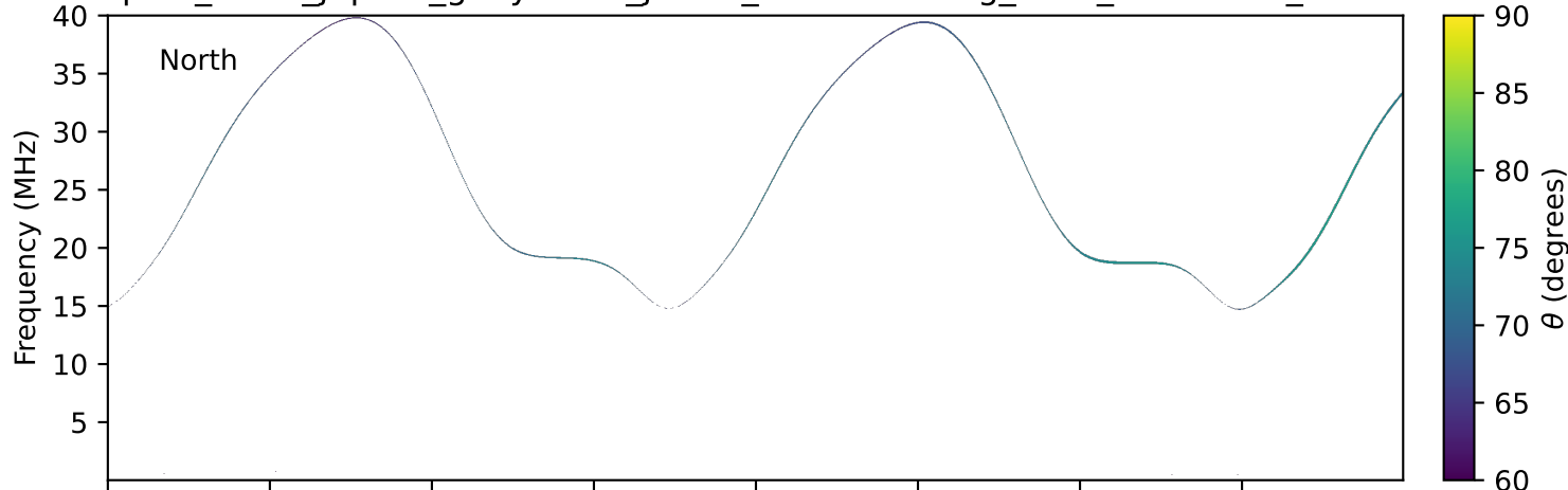
expres_earth_jupiter_ganymede_jrm33_lossc-wid1deg_3kev_20270320_v11.cdf
