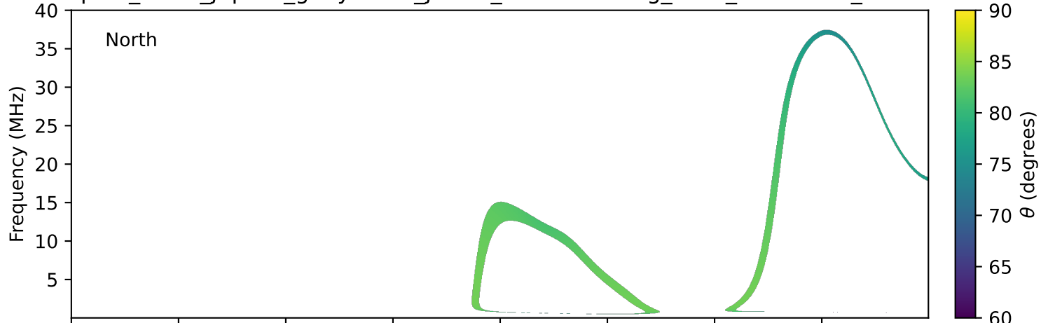
expres_earth_jupiter_ganymede_jrm33_lossc-wid1deg_3kev_20270318_v11.cdf
