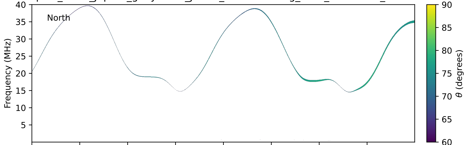
expres_earth_jupiter_ganymede_jrm33_lossc-wid1deg_3kev_20270306_v11.cdf
