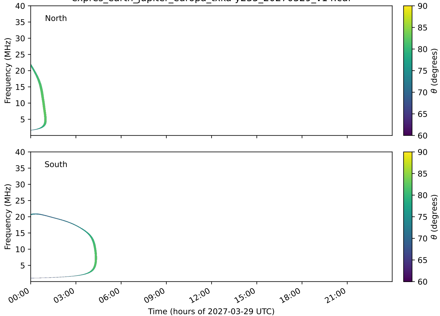
expres_earth_jupiter_europa_txka-y235_20270329_v14.cdf
