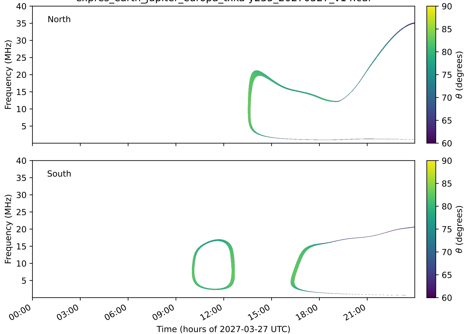
expres_earth_jupiter_europa_txka-y235_20270327_v14.cdf
