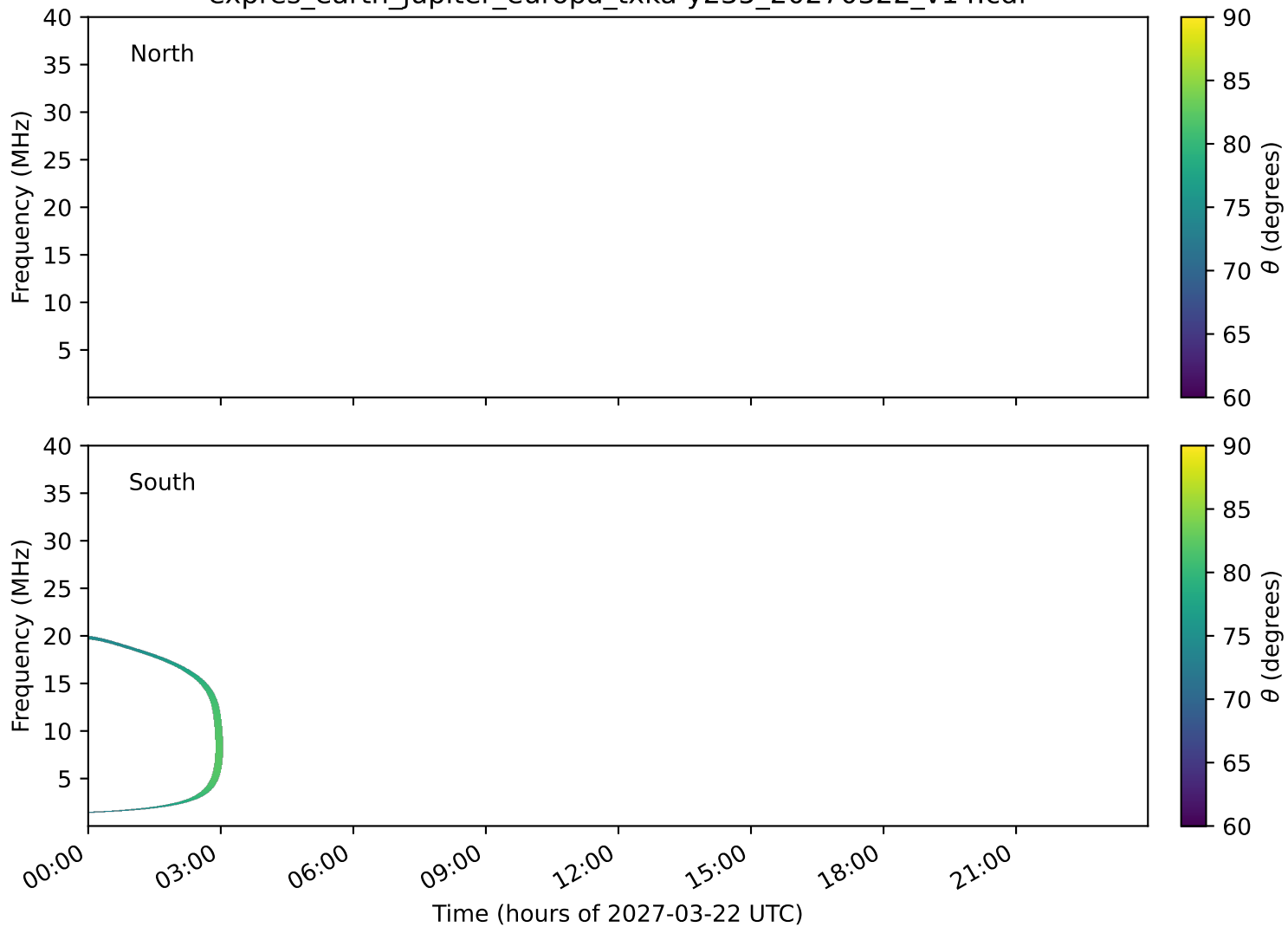
expres_earth_jupiter_europa_txka-y235_20270322_v14.cdf
