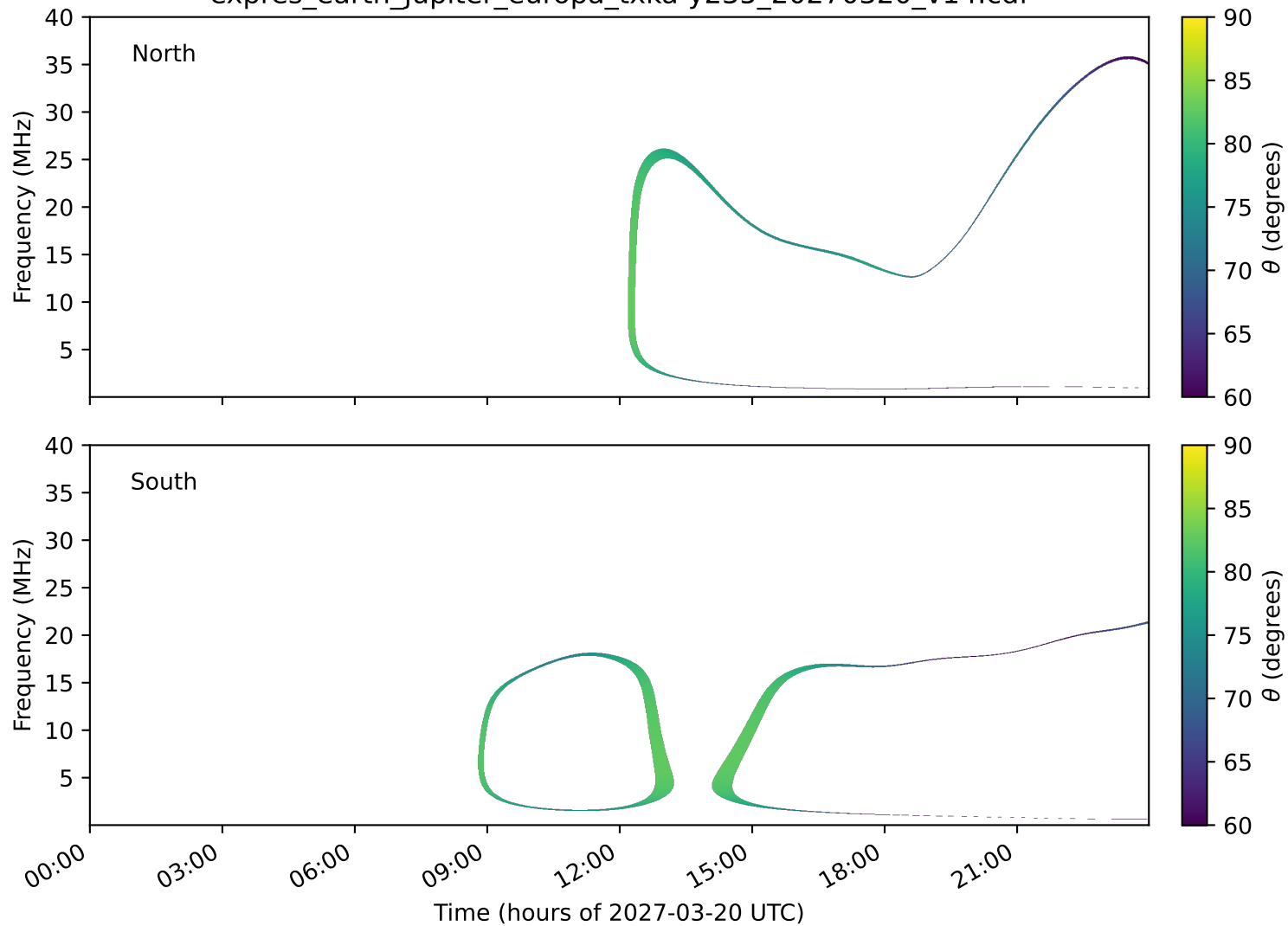
expres_earth_jupiter_europa_txka-y235_20270320_v14.cdf
