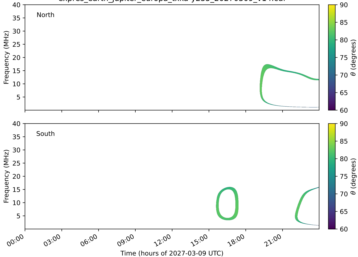
expres_earth_jupiter_europa_txka-y235_20270309_v14.cdf
