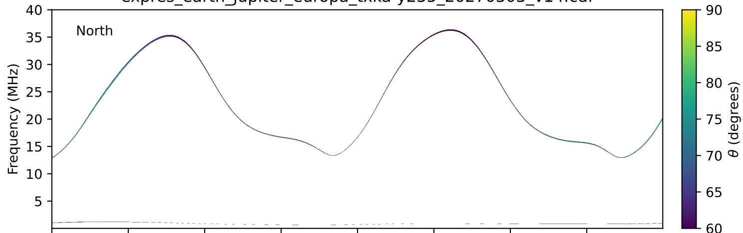
expres_earth_jupiter_europa_txka-y235_20270303_v14.cdf
