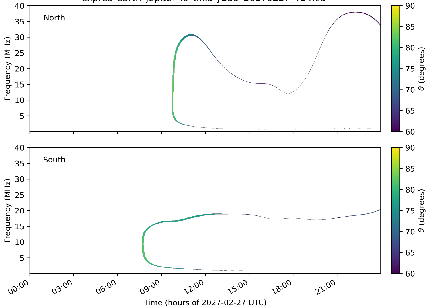
expres_earth_jupiter_io_txka-y235_20270227_v14.cdf
